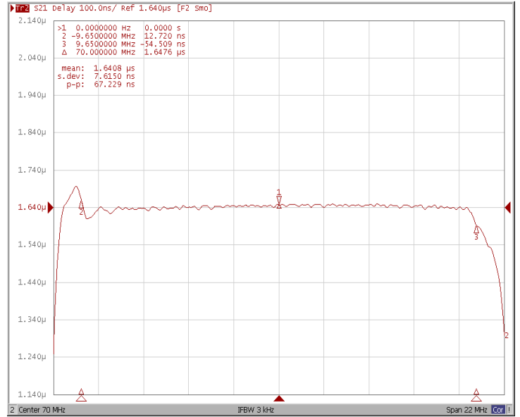
Group Delay Variation Fo \pm 9.65\text{MHz}
