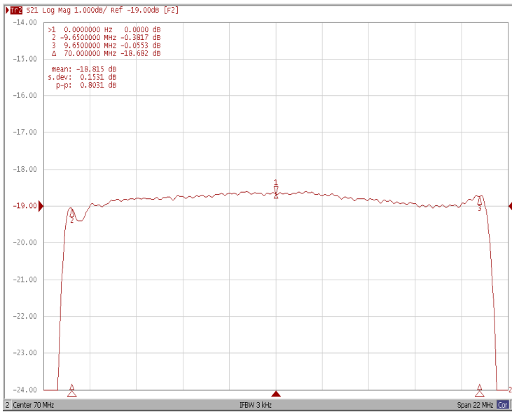
Ripple Variation Fo \pm 9.65\text{MHz}
